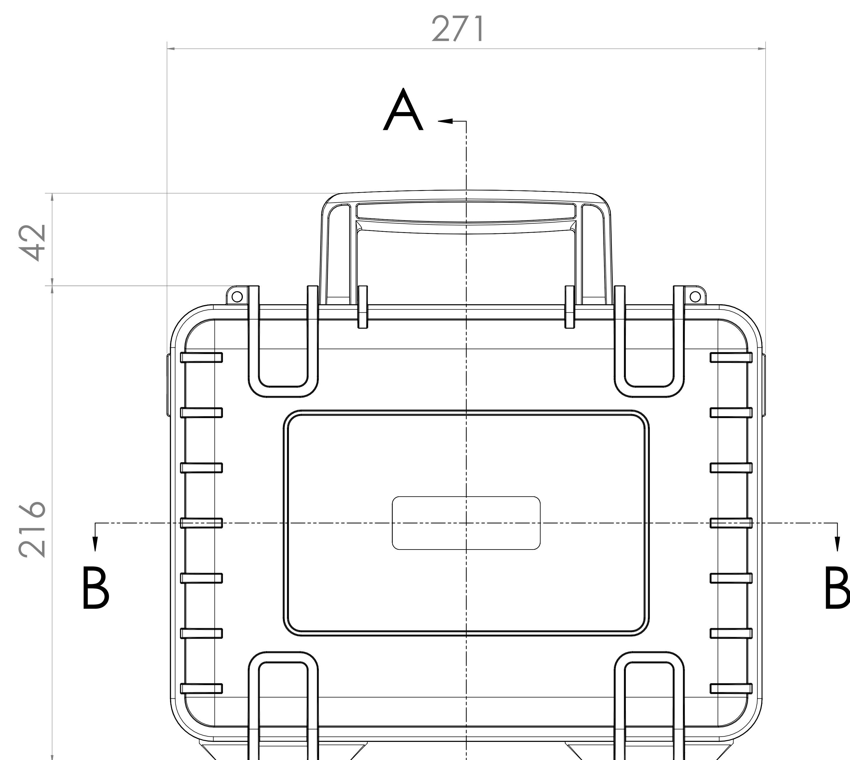
top view
