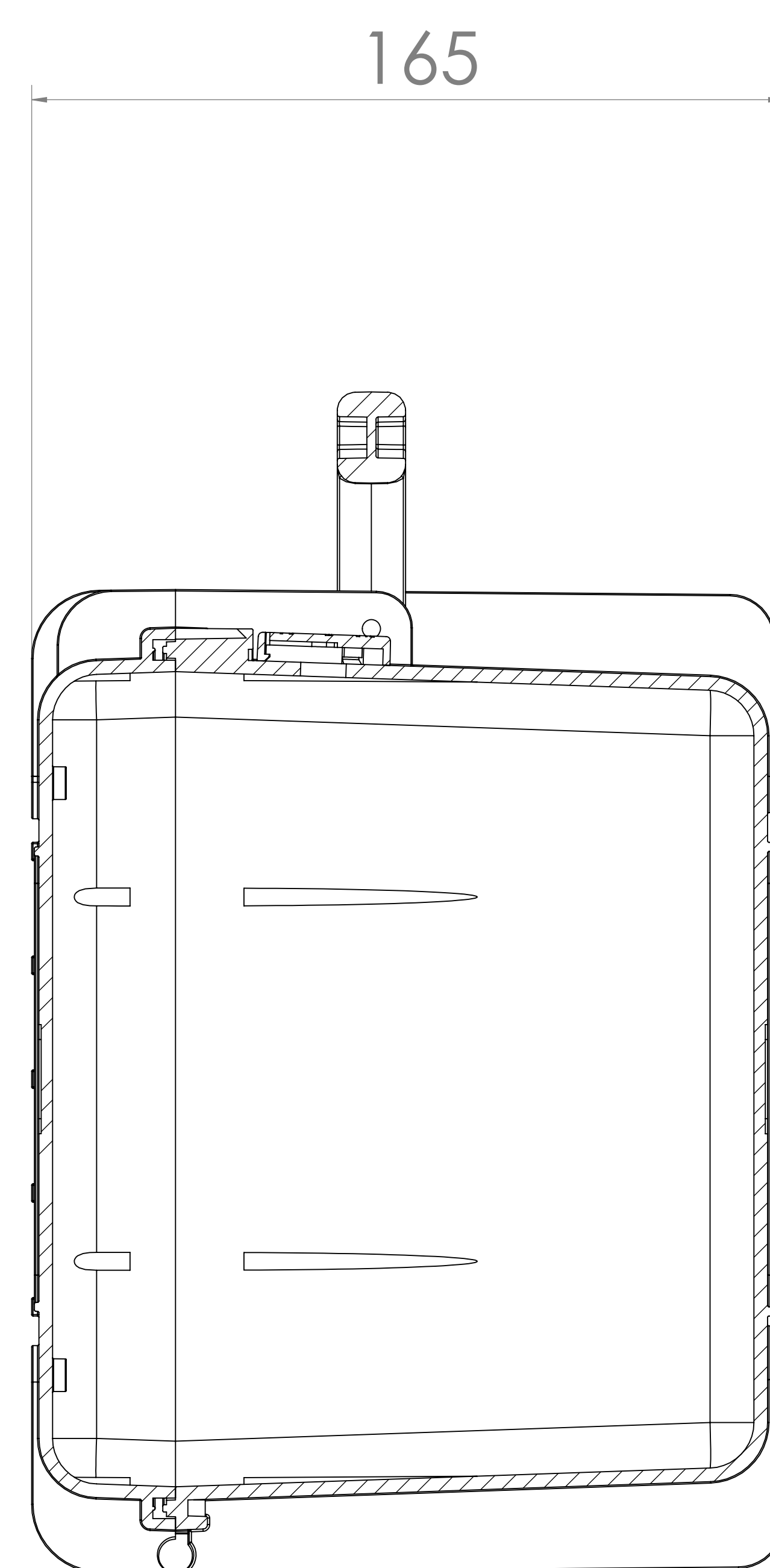
side view
